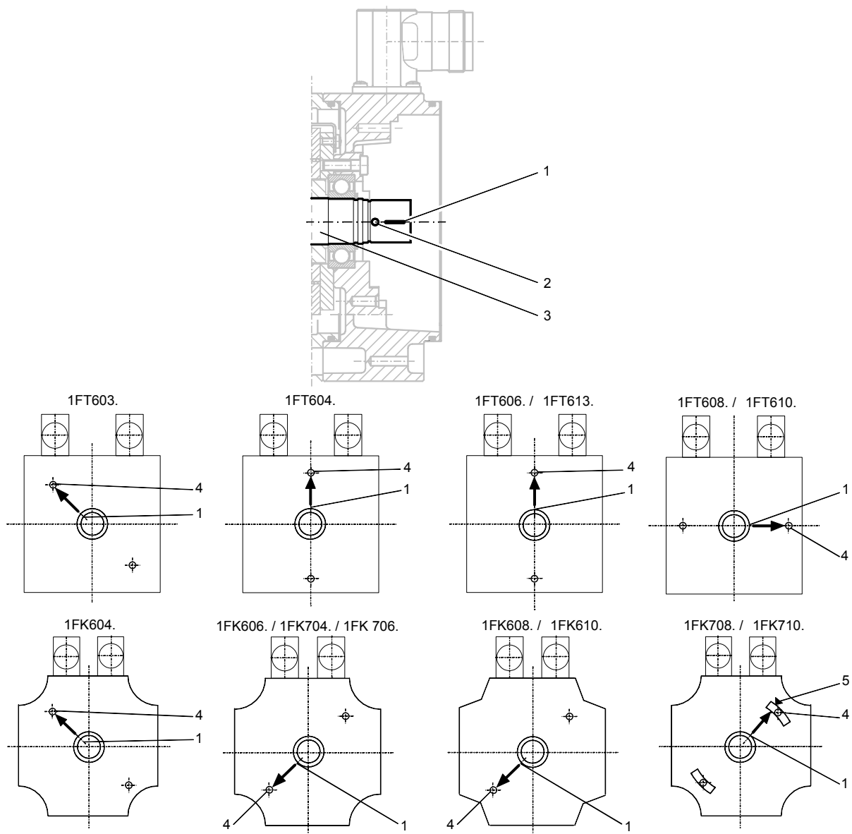
Figure 12 Aligning the motor shaft
