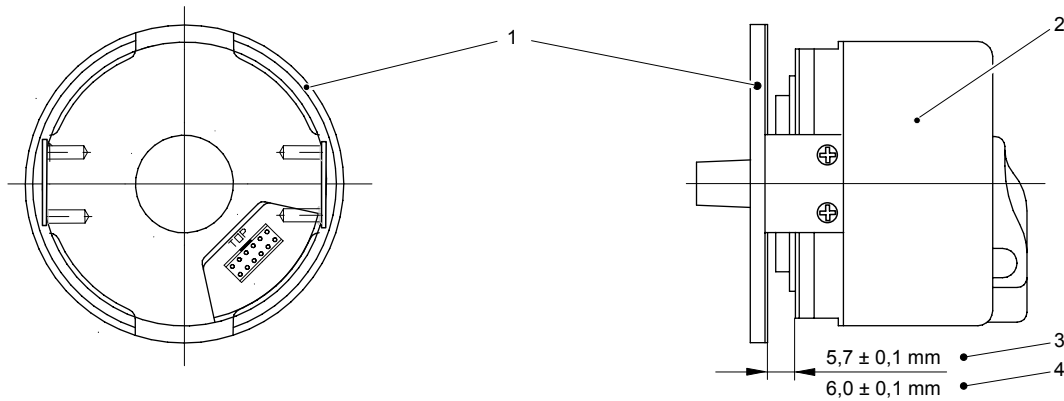
Figure 8 Assembly of motor 1FK604.
