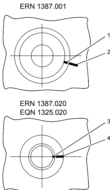
Figure 13 Aligning the encoder
