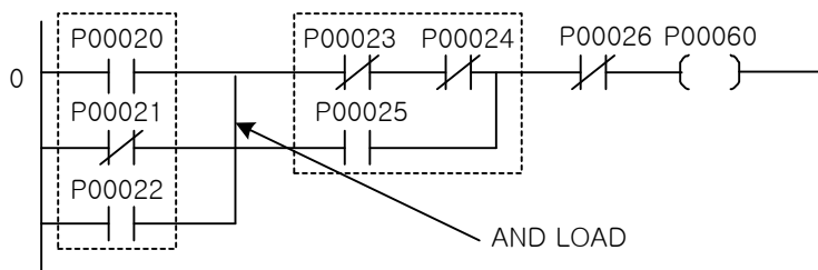
[Ladder Program]
